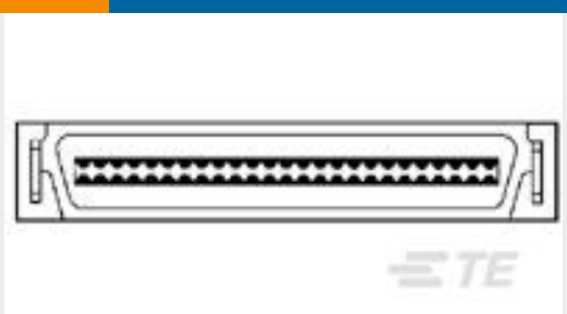
TE Part #1-1734101-1 Champ050 series,100pos,Au over PdNi
