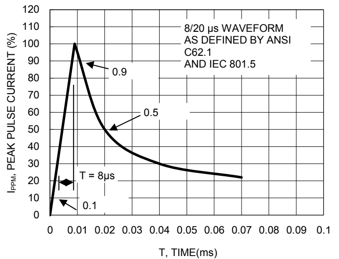
Fig12. Pulse Waveform
