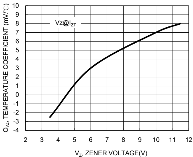
Fig3. Zener Voltage – To 12 Voltages
