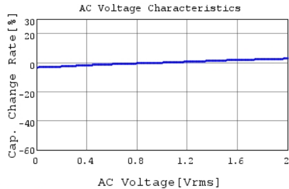
GRT033R61E151KE01 C-AC Voltage capchange, DC
