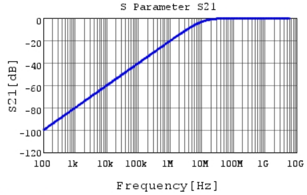
GRT033R61E151KE01 S21 DCOV,25degC
