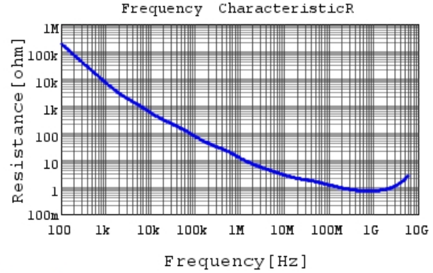
GRT033R61E151KE01 R DCOV, 25degC
