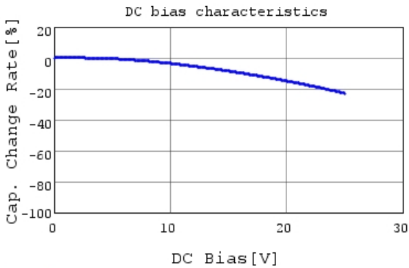
GRT033R61E151KE01 C-DC bias capchange, 25.0c
