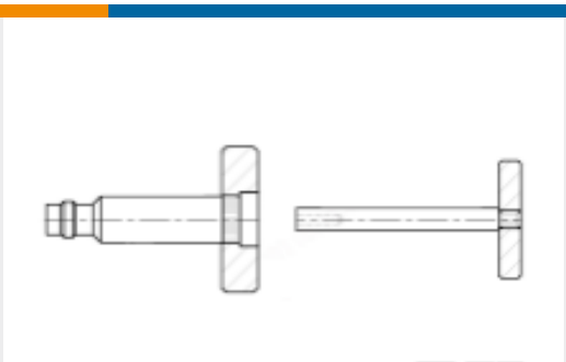
TE Part #1055447-1 OSM PLUG DIELECTRIC INSERT TL
