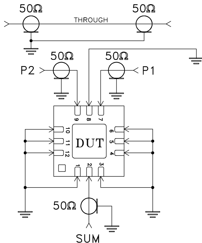
Schematic Diagram
