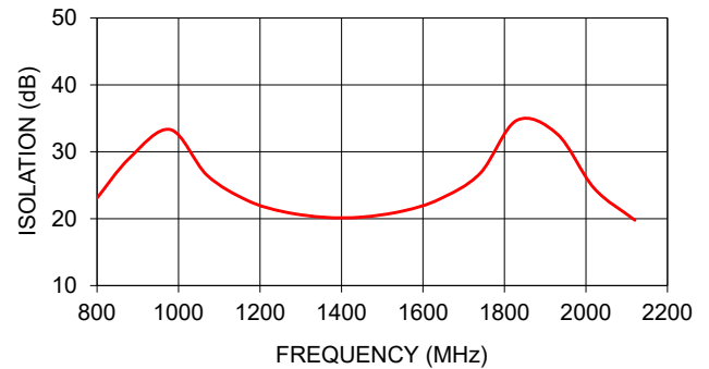
GP2S+ ISOLATION
