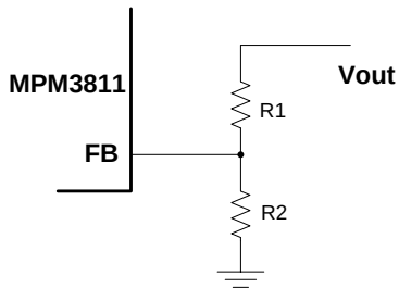
Figure 3: Feedback Network
