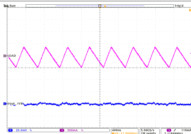
Figure 8-34. PSM Operation
