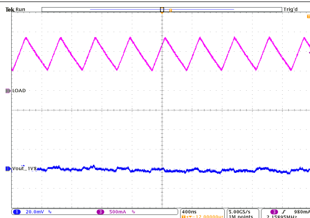
Figure 8-33. PWM Operation
