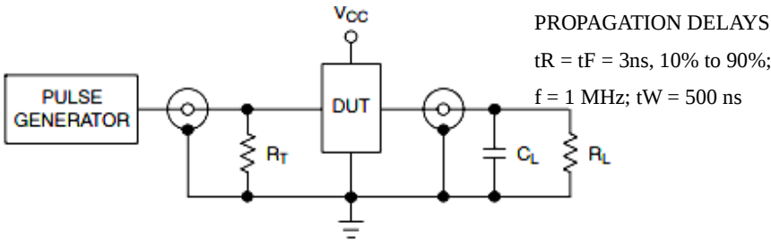
Figure 4. Test Circuit
