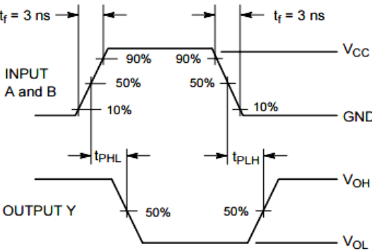
Figure 3. Switching Waveform
