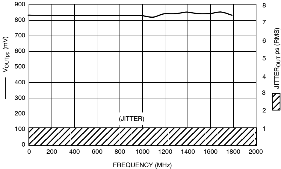
Figure 6. \div 2, F_{max}/Jitter
