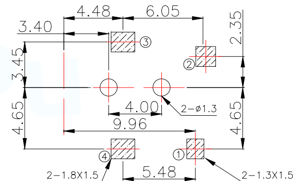
PCB.WELDING DRAWING (TOLERANCE:±0.05)
