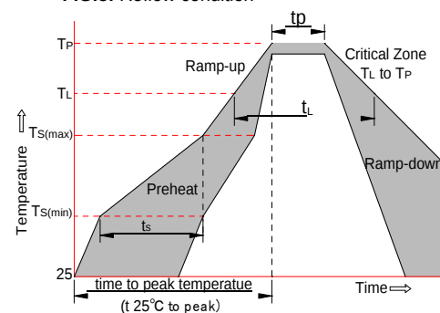
FIG.5: Reflow condition
