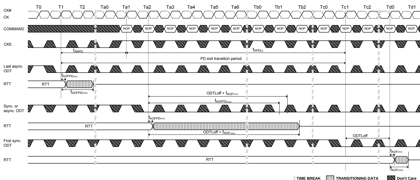
Figure 76. Transition period for short CKE cycles, entry and exit period overlapping (AL = 0, WL = 5, tANPD = WL - 1 = 4)
