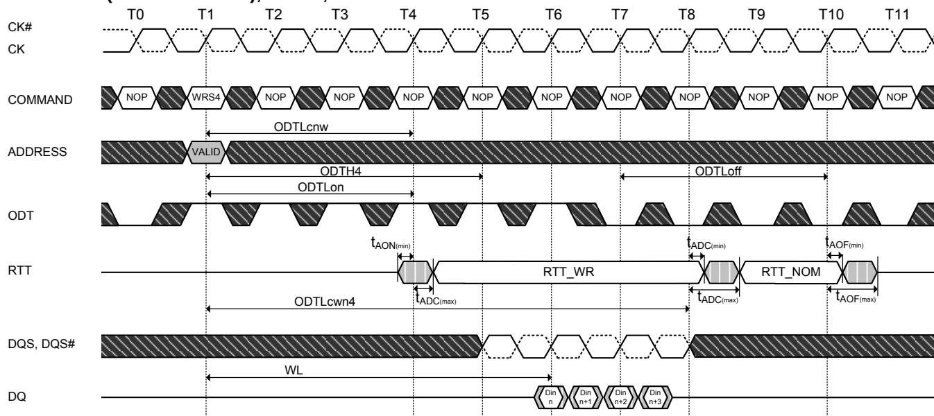
Figure 70. Dynamic ODT: Behavior with ODT pin being asserted together with write command for a duration of 6 clock cycles, example for BC4
