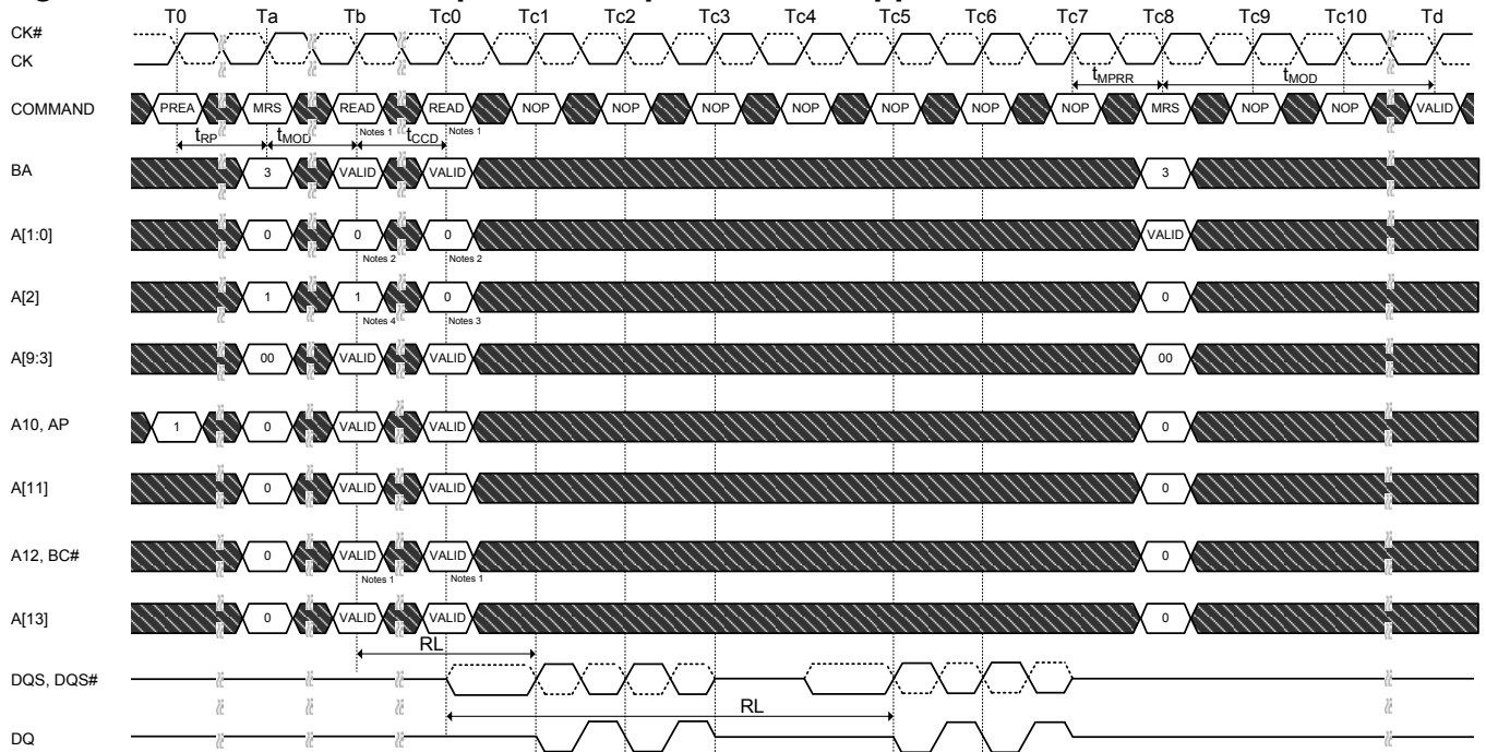
Figure 28. MPR Readout of predefined pattern,BC4 upper nibble then lower nibble
