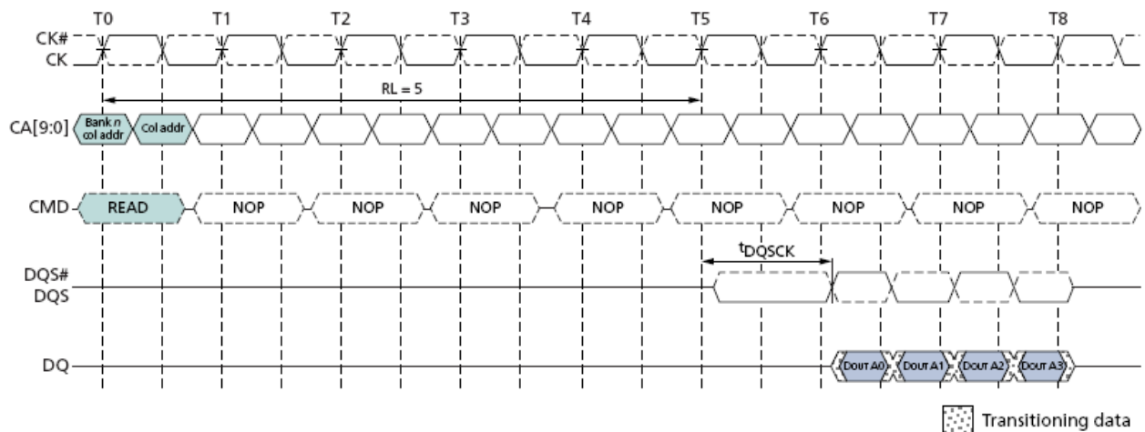
Burst Read: RL=5, BL=4, T_{dqsck} > T_{ck}
