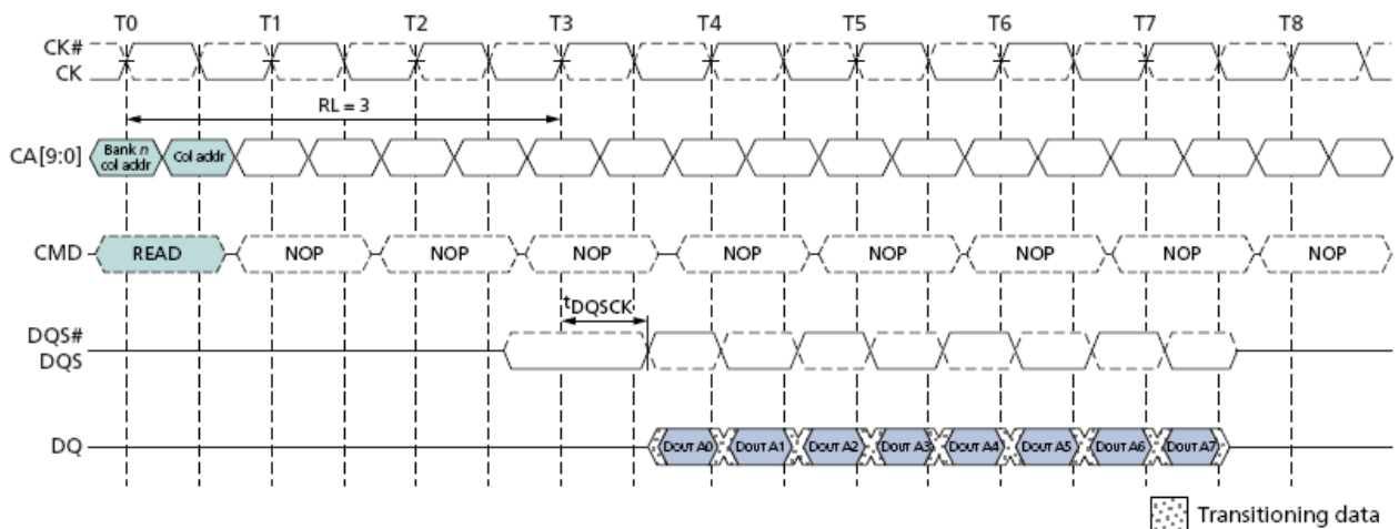
Burst Read: RL=3, BL=8, T_{dqsck} < T_{ck}
