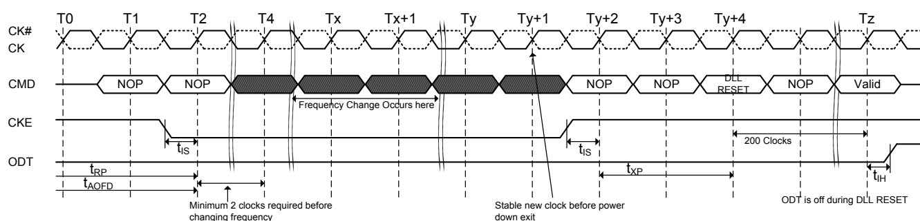
Figure 62. Clock frequency change in precharge power down mode
