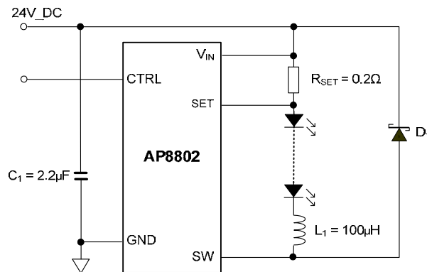
Figure. 14 Typical Application Circuit for I_{LED} = 1\text{A}
