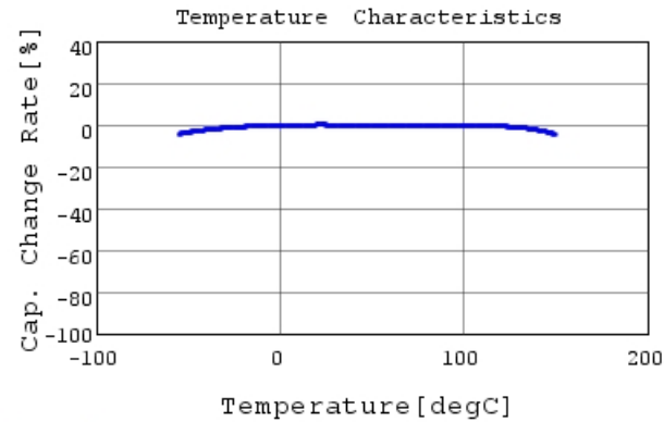
GCJ188R92A123KA01 C-Temp. capchange, DC0.0V,
