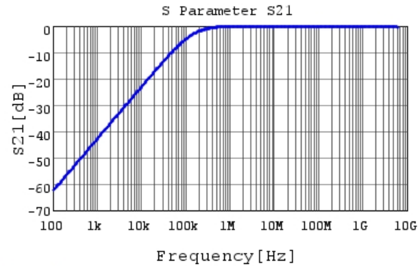
GCJ188R92A123KA01 S21 DC0V,25degC
