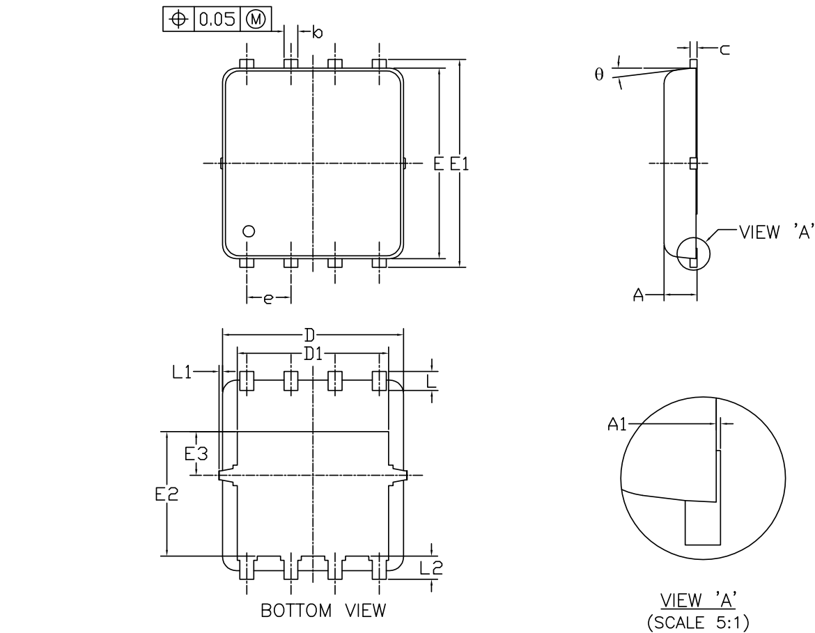
DFN5x6_8L_EP1_P PACKAGE OUTLIN
