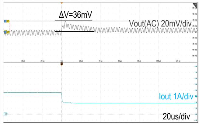
( V_{IN} = 24.0V , C_{OUT} = 110\mu F , I_{OUT} = 3.5A to 1.75A , 1A/\mu s ) Figure 28. Step Load Transient Response
