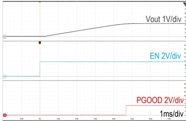
( V_{IN} = 24.0V , I_{OUT} = 3.5A , C_{OUT} = 110\mu F ) Figure 13. On/Off Enable Waveform
