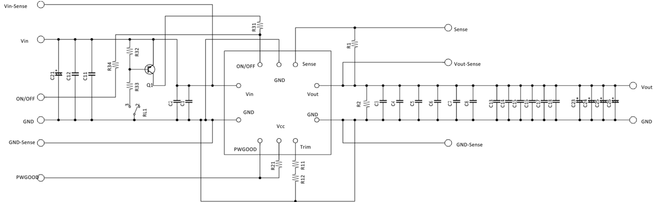
Figure 34. Application Circuit
