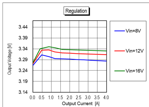
Figure 6. V_{OUT} vs. Load Current and Line Voltage
