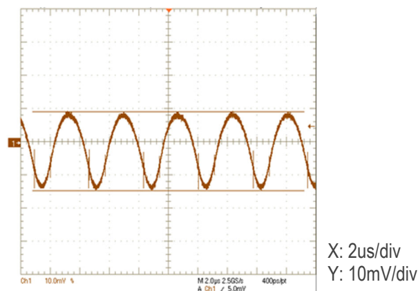
( V_{IN} = 12\text{V} , I_{OUT} = 4.0\text{A} , C_{OUT} = 110\mu\text{F} , ScopeBW = 20MHz) Figure 8. Output Ripple and Noise
