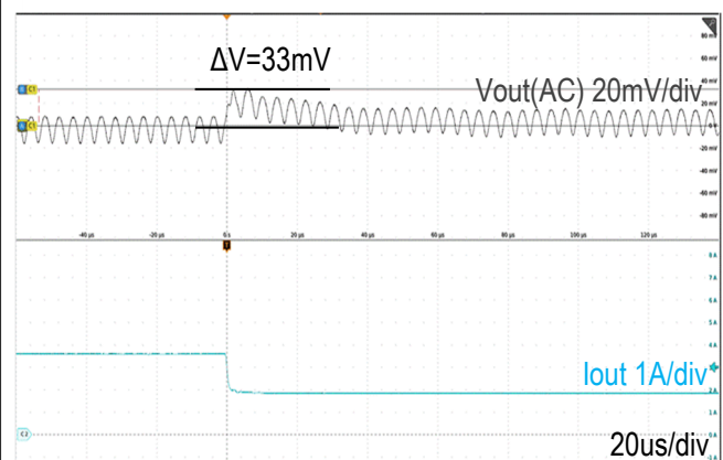
( V_{IN} = 24.0V , C_{OUT} = 110\mu F , I_{OUT} = 3.5A to 1.75A , 1A/us ) Figure 16. Step Load Transient Response
