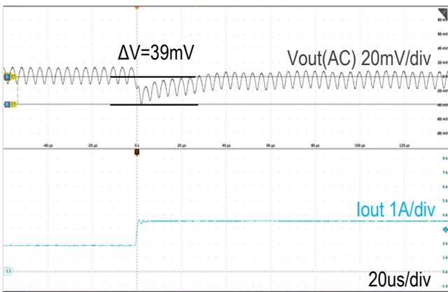
( V_{IN} = 24.0V , C_{OUT} = 110\mu F , I_{OUT} = 1.75A to 3.5A , 1A/us ) Figure 15. Step Load Transient Response
