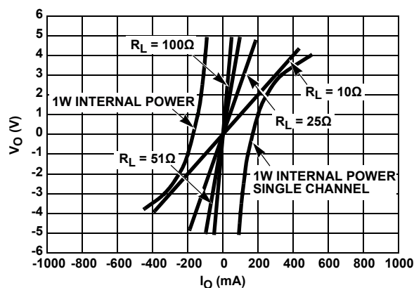
FIGURE 22. OUTPUT VOLTAGE AND CURRENT LIMITATIONS
