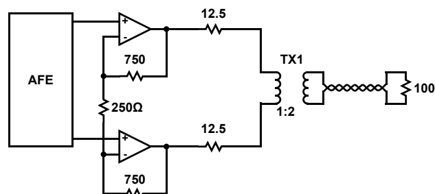
FIGURE 24. CIRCUIT CONFIGURATION
