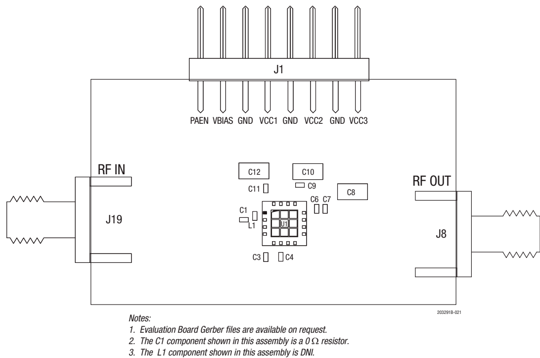
Figure 21. Evaluation Board Assembly Drawing
