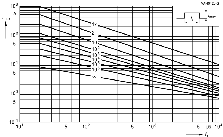
SIOV-S10K11 ... K40E2
