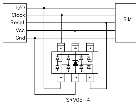
Figure 6 - SIM Port
