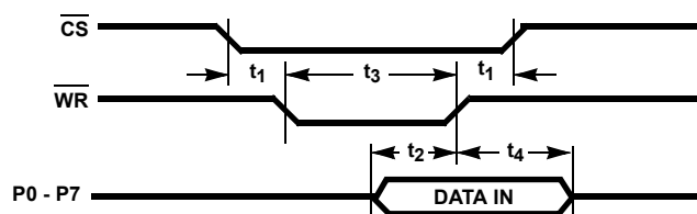
FIGURE 1A. WRITE
