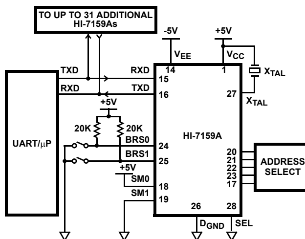
FIGURE 4C. SERIAL MODE 2
