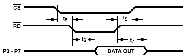
FIGURE 1D. READ
