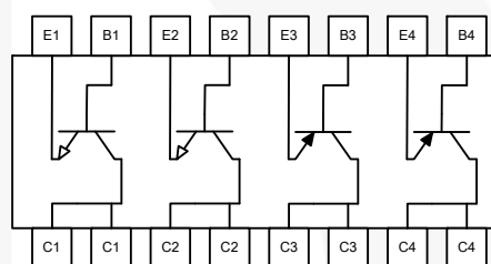
Figure 2. Internal Connection
