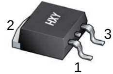
TO-252-2L (TO-252-2(DPAK))
