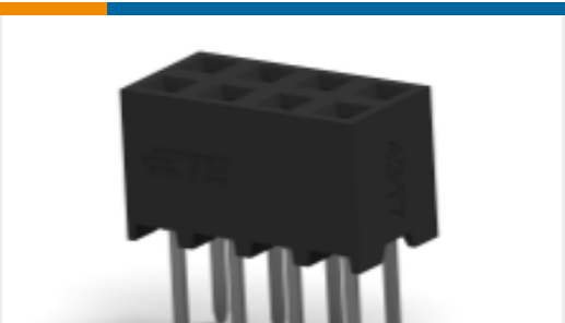
TE Part #2314814-8 8P, 2MM, B-B, REC, DRV, 2.0, 0.76 AU, TB, W/CAP
