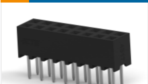
TE Part #1-2314812-6 16P, 2MM, B-B, REC, DRV, 2.0, 0.1 AU, TB, W/CAP
