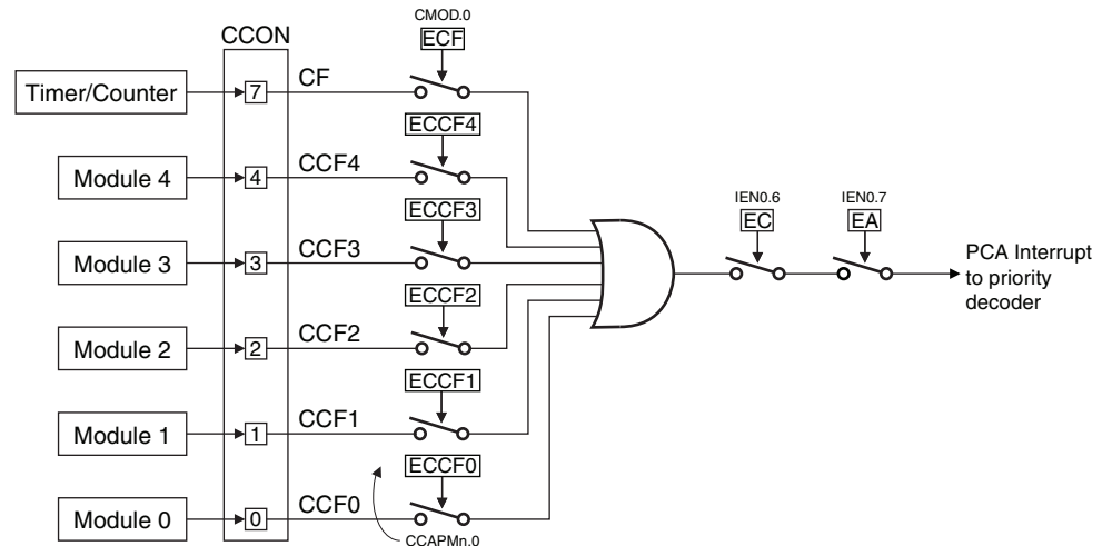
Figure 14-2. PCA Interrupt System
