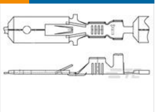
TE Part #444152-2 FF 250 TAB 1-5 MM2 .39X13.2 ELECTRO TPBR
