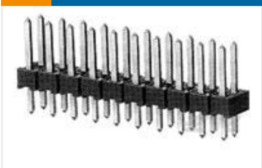
TE Part #5-146257-3 06 MODII HDR DRST B/A .100CL LF
