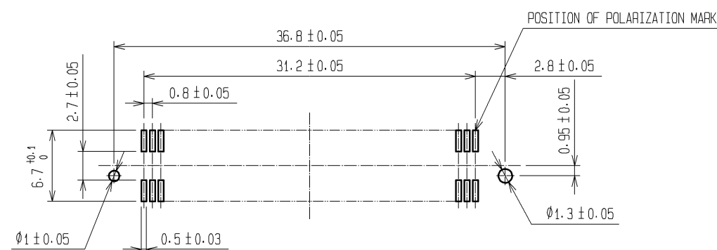
RECOMMENDED LAND PATTERN DIMENSION OF PCB(MOUNTING SIDE)
