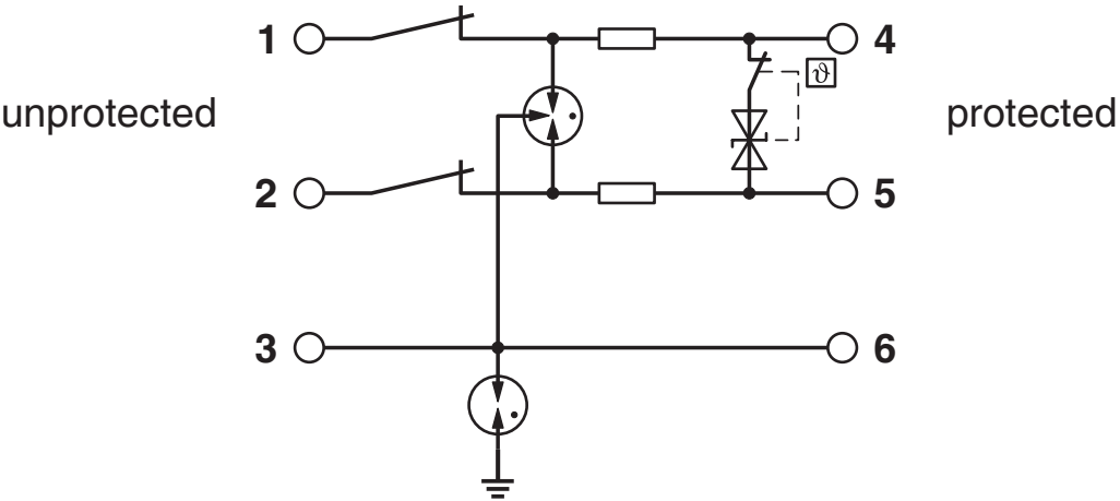
Circuit diagram
