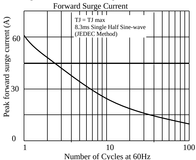
Fig. 2 - Maximum Non-repetitive Peak
