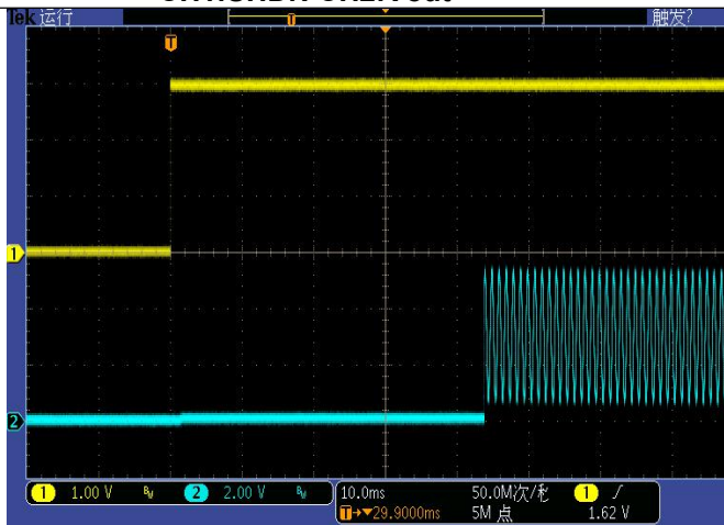
AGC Start-up Waveform
