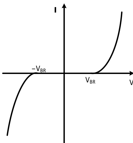
Figure 4. Bidirectional TVS tube without Snapback characteristics I/V
