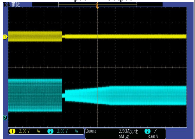
AGC Shut-down Waveform
