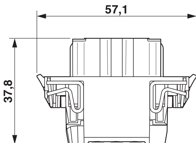
Dimensional drawing
