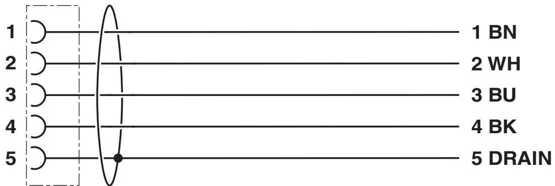
Circuit diagram
