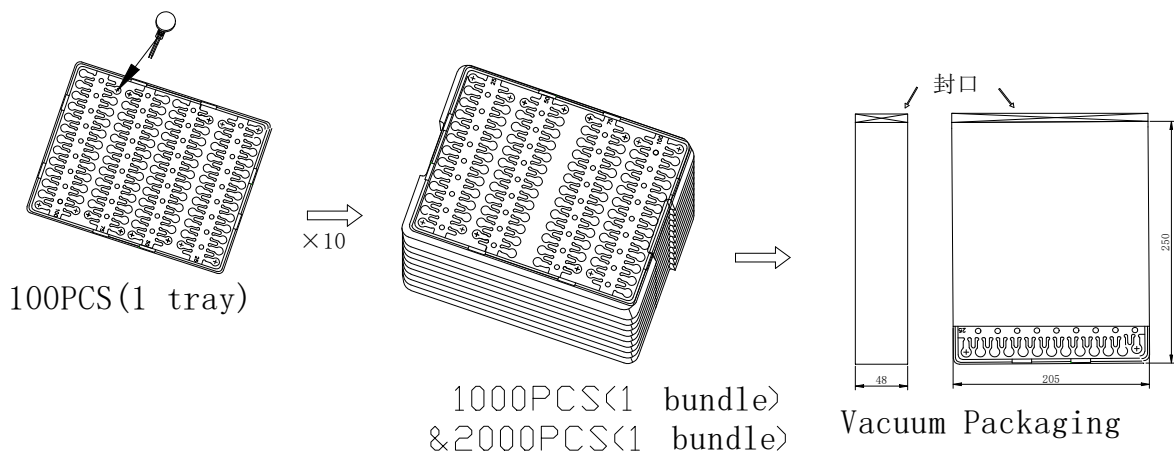
Pack drawing of Vibrator Motor
