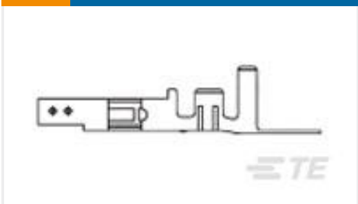
TE Part #52935-3 TERMINAL,PIDG SPR SPD 16-14 6
