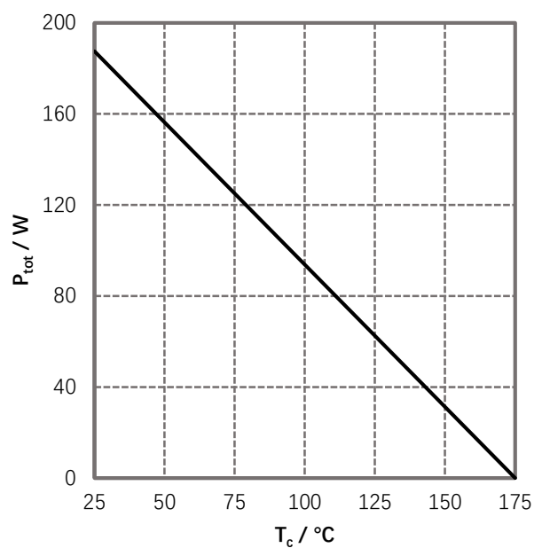
Figure 3. Power Derating
