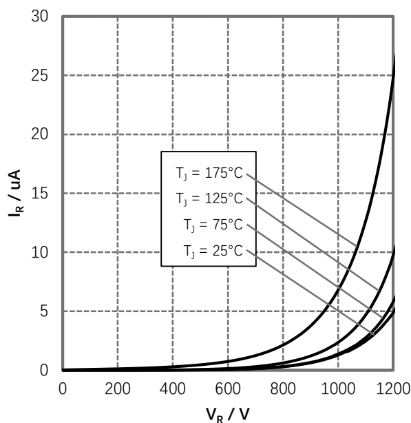
Figure 2. Reverse Characteristics
