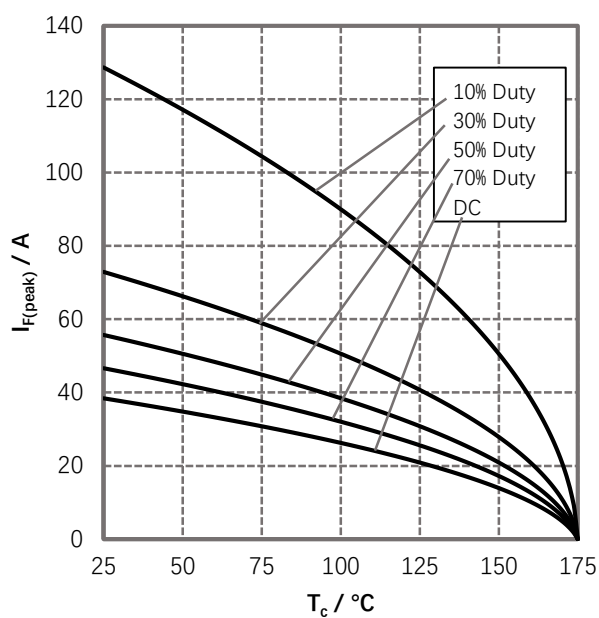
Figure 4. Current Derating
