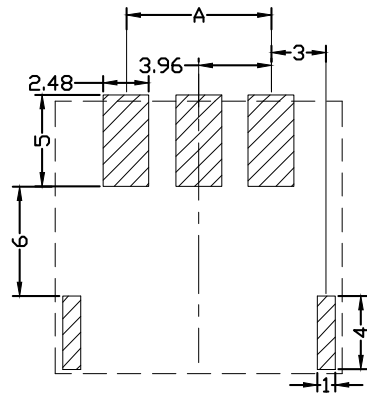
SUGGESTED PCB LAYOUT (COMPONENT SIDE)
