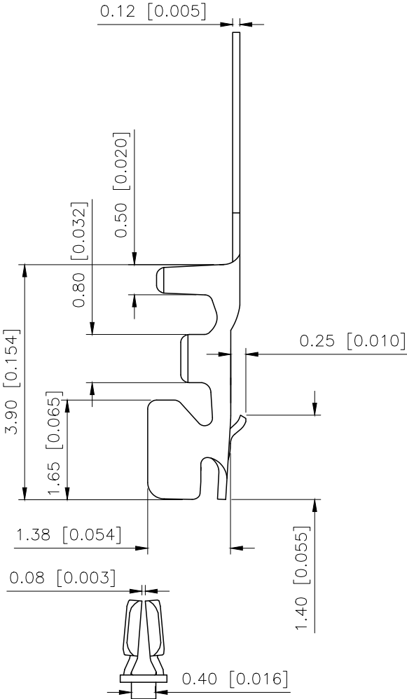
SEC:C-C
