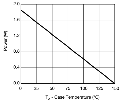
Power, Junction-to-Ambient
