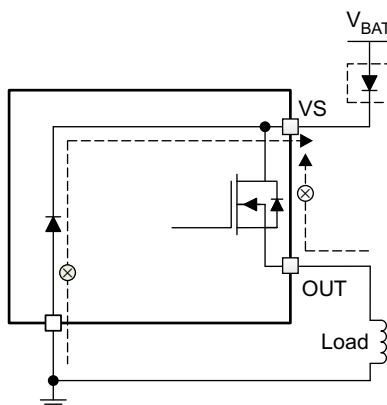
Figure 34. Reverse-Current External Protection, Method 1
