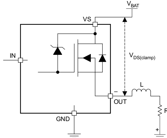
Figure 26. Drain-to-Source Clamping Structure
