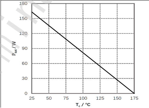
Figure 4. Power Dissipation
