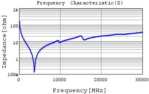
GJM0335G2A9R9WB01 |Z| DCOV, 25degC
