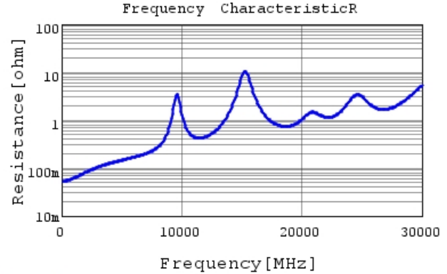
GJM0335G2A9R9WB01 R DCOV, 25degC
