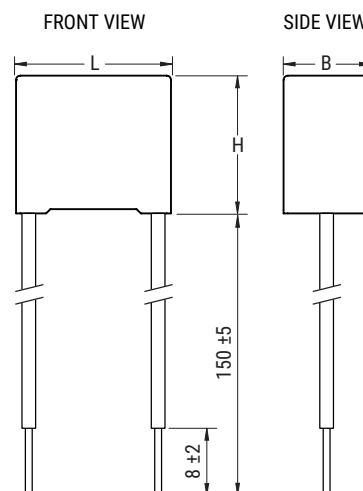
Insulated Flexible Leads 0.5 mm 2
