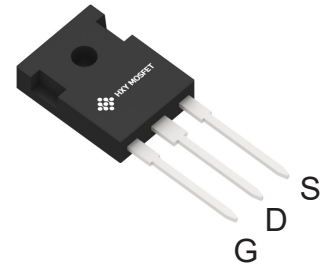
TO-247
