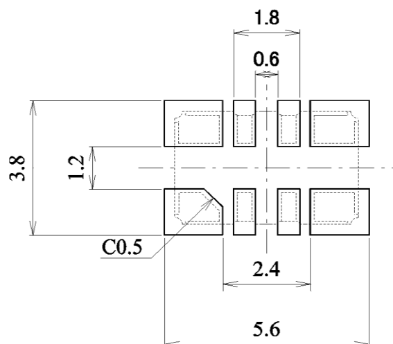
Recomended land pattern (Top View)
