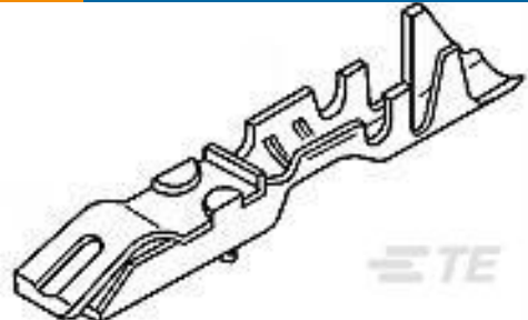
TE Part #87124-1 LOCKING CLIP CONT ASSY .025 SQ
