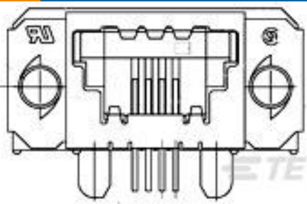
TE Part #5-1761185-1 4 SDL SE GRND RCPT ASSY
