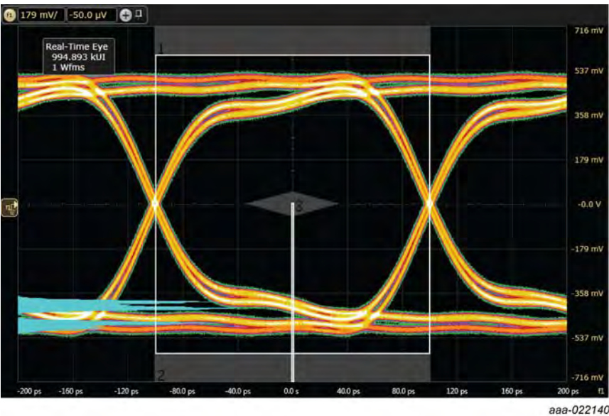
Fig 7. USB 3.1 eye diagram, test board with PCMF2USB30; typical values
