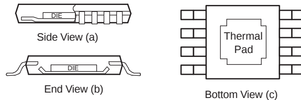
Figure 79. Views of Thermally-Enhanced Package
